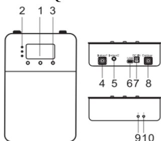
Triband/Quintband Booster
