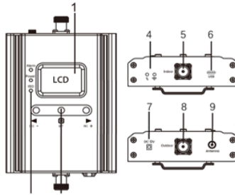
Dualband Booster
