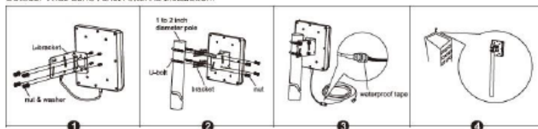
Outdoor Wide Band Panel Antenna Installation:
